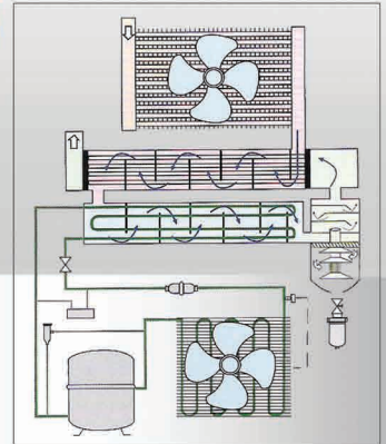
Air Cooling Flow Chart
